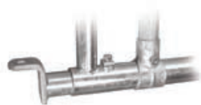
Adjustable, swiveling and raisable end-piece
